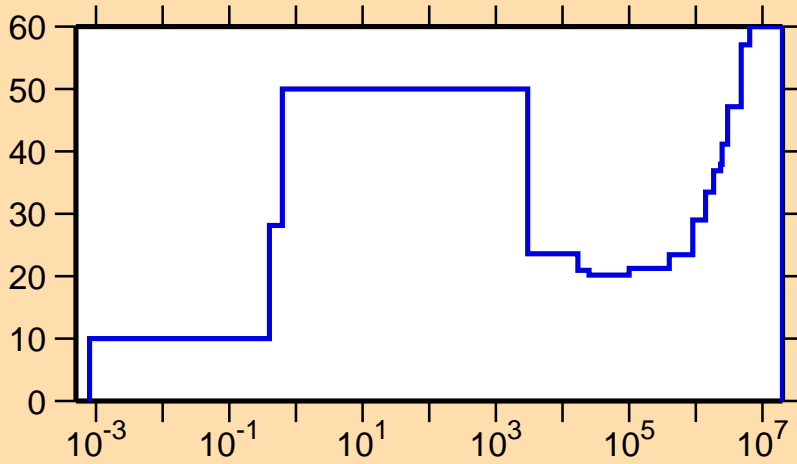
\Delta\sigma/\sigma vs. E for ^{134}\text{Xe}(n,\gamma)
