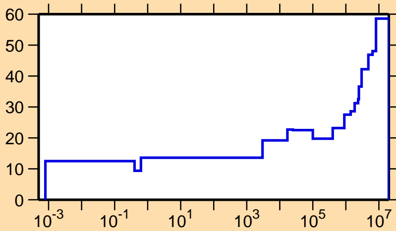
\Delta\sigma/\sigma vs. E for ^{108}\text{Pd}(n,\gamma)
