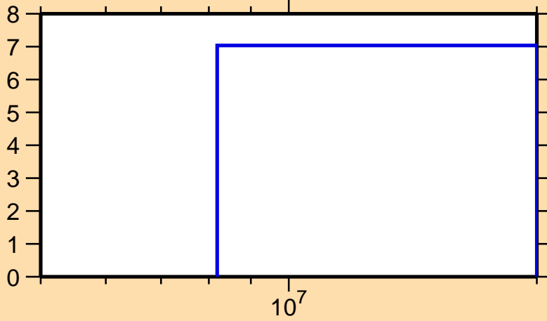
\Delta\sigma/\sigma vs. E for ^{108}\text{Pd}(n,2n)
