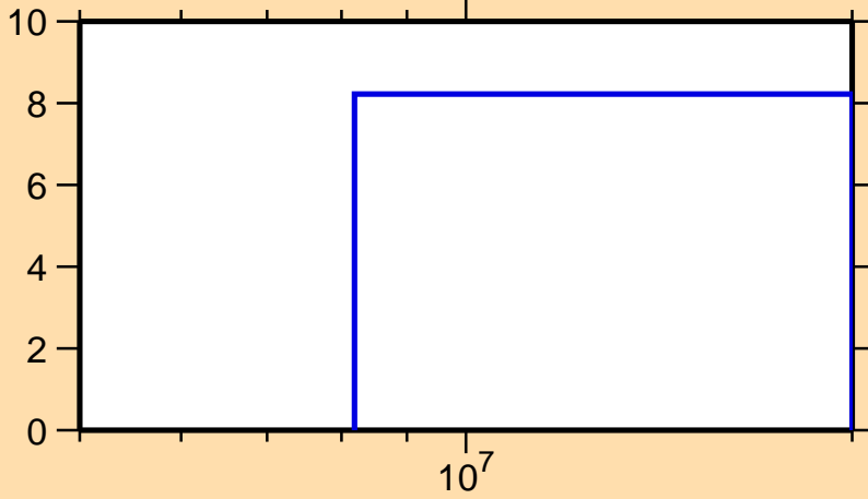
\Delta\sigma/\sigma vs. E for ^{106}\text{Pd}(n,2n)
