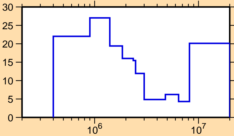
\Delta\sigma/\sigma vs. E for ^{106}\text{Pd}(n,\text{inel.})
