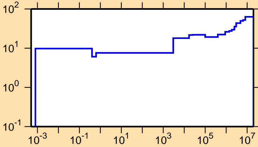
\Delta\sigma/\sigma vs. E for ^{106}\text{Pd}(n,\gamma)
