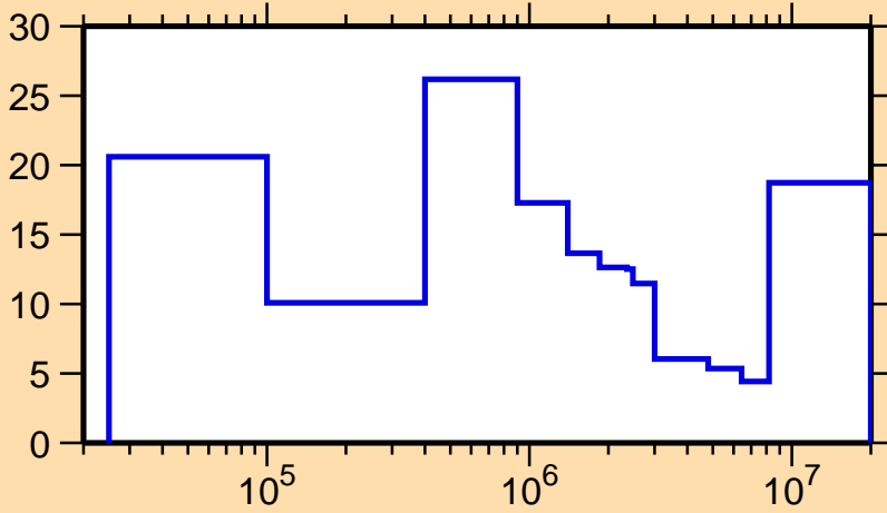
\Delta\sigma/\sigma vs. E for ^{103}\text{Rh}(n,\text{inel.})
