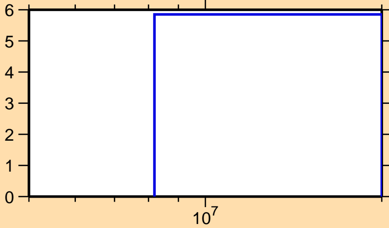
\Delta\sigma/\sigma vs. E for ^{104}\text{Ru}(n,2n)
