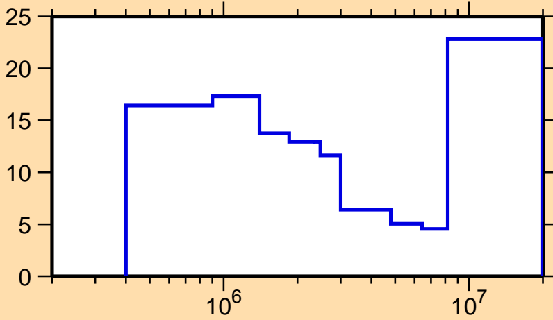
\Delta\sigma/\sigma vs. E for ^{102}\text{Ru}(n,\text{inel.})
