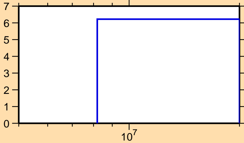
\Delta\sigma/\sigma vs. E for ^{102}\text{Ru}(n,2n)
