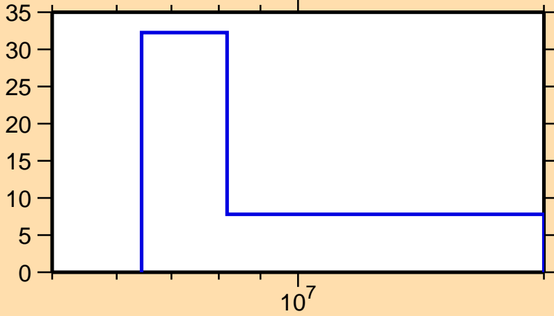
\Delta\sigma/\sigma vs. E for ^{101}\text{Ru}(n,2n)
