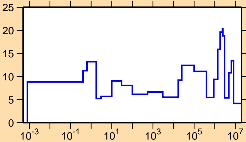
\Delta\sigma/\sigma vs. E for ^{99}\text{Tc}(n,\text{el.})
