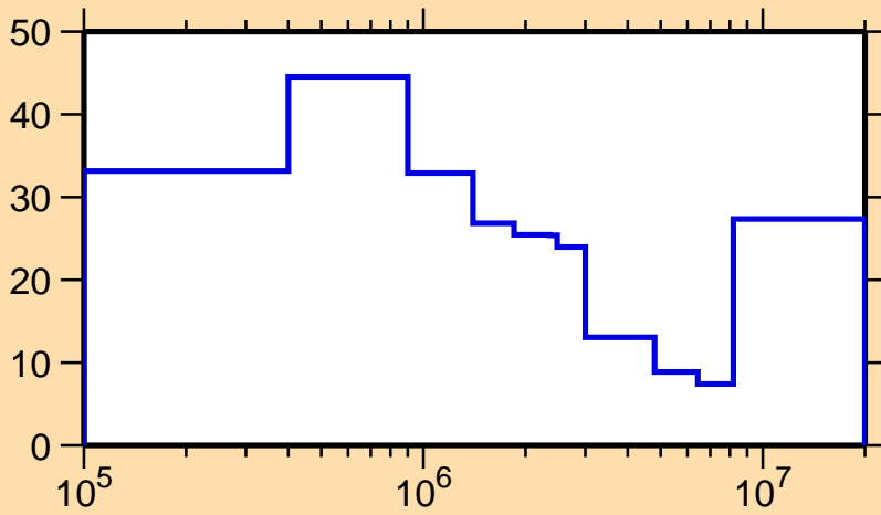
\Delta\sigma/\sigma vs. E for ^{99}\text{Tc}(n,\text{inel.})
