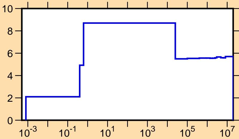
\Delta\sigma/\sigma vs. E for ^{100}\text{Mo}(n,\text{tot.})
