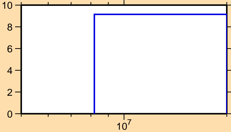
\Delta\sigma/\sigma vs. E for ^{100}\text{Mo}(n,2n)
