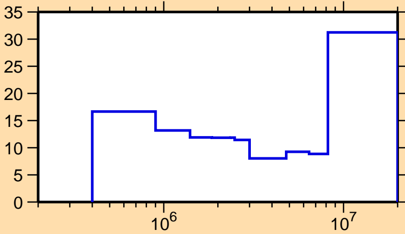
\Delta\sigma/\sigma vs. E for ^{100}\text{Mo}(n,\text{inel.})
