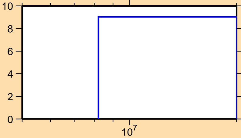
\Delta\sigma/\sigma vs. E for ^{98}\text{Mo}(n,2n)
