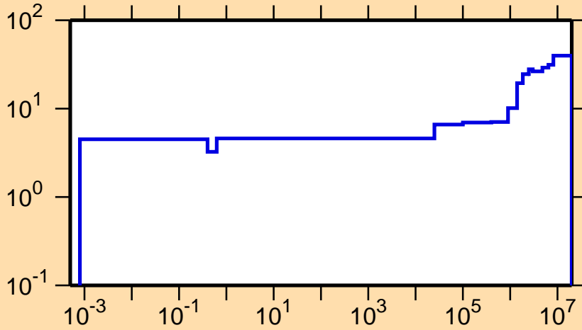
\Delta\sigma/\sigma vs. E for ^{98}\text{Mo}(n,\gamma)
