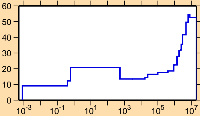
\Delta\sigma/\sigma vs. E for ^{97}\text{Mo}(n,\gamma)
