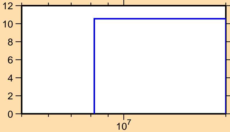
\Delta\sigma/\sigma vs. E for ^{96}\text{Mo}(n,2n)
