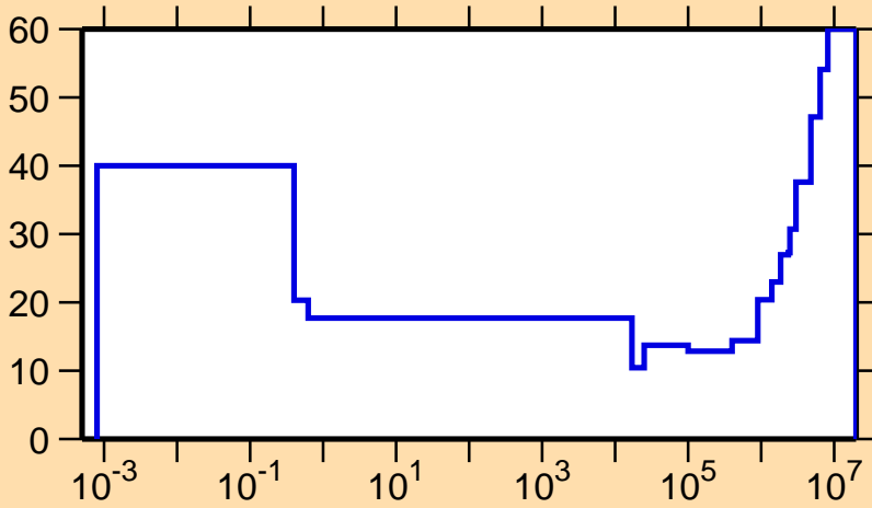
\Delta\sigma/\sigma vs. E for ^{96}\text{Mo}(n,\gamma)
