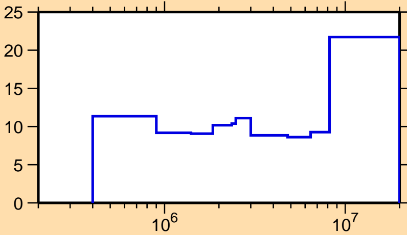
\Delta\sigma/\sigma vs. E for ^{96}\text{Mo}(n,\text{inel.})
