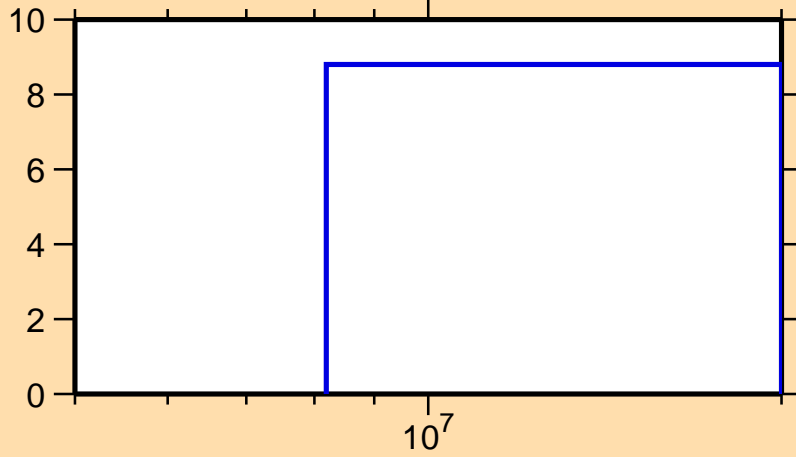
\Delta\sigma/\sigma vs. E for ^{94}\text{Mo}(n,2n)
