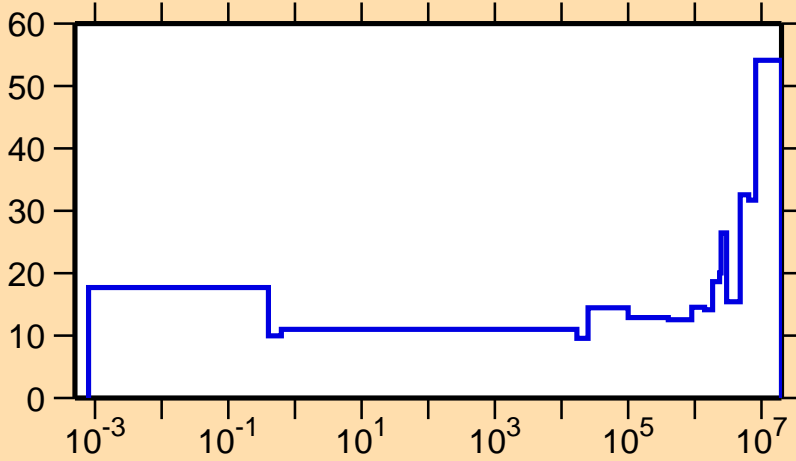
\Delta\sigma/\sigma vs. E for ^{94}\text{Mo}(n,\gamma)
