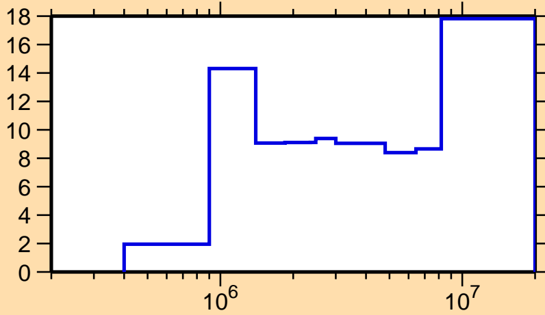
\Delta\sigma/\sigma vs. E for ^{94}\text{Mo}(n,\text{inel.})
