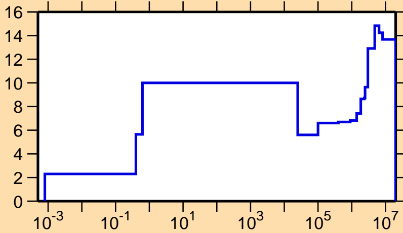
\Delta\sigma/\sigma vs. E for ^{92}\text{Mo}(n,\text{el.})
