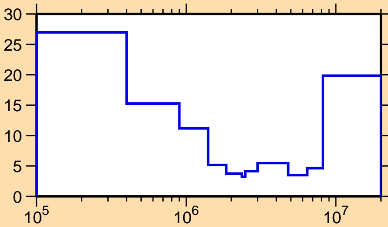
\Delta\sigma/\sigma vs. E for ^{95}\text{Nb}(n,\text{inel.})
