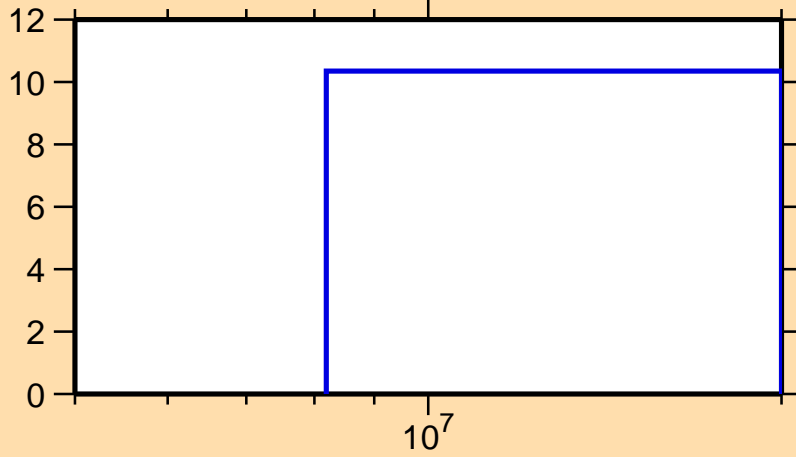
\Delta\sigma/\sigma vs. E for ^{95}\text{Nb}(n,2n)
