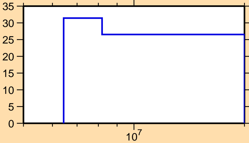
\Delta\sigma/\sigma vs. E for ^{95}\text{Zr}(n,2n)
