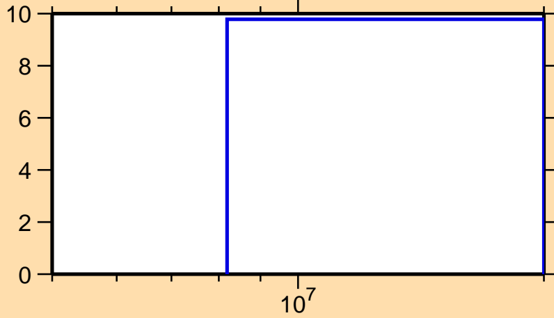
\Delta\sigma/\sigma vs. E for ^{94}\text{Zr}(n,2n)
