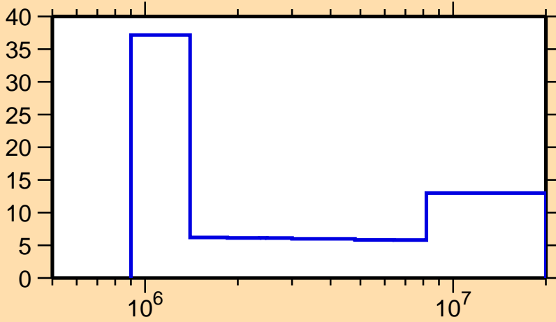
\Delta\sigma/\sigma vs. E for ^{94}\text{Zr}(n,\text{inel.})
