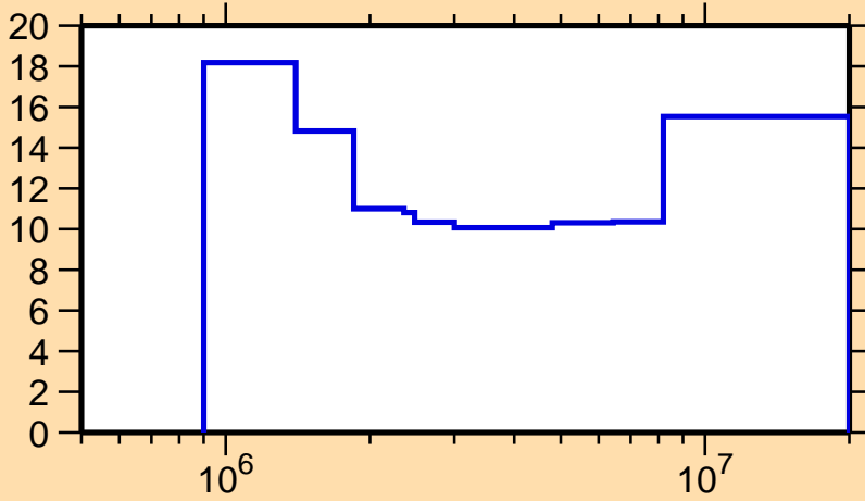
\Delta\sigma/\sigma vs. E for ^{91}\text{Zr}(n,\text{inel.})
