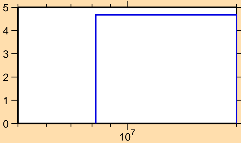
\Delta\sigma/\sigma vs. E for ^{50}\text{Cr}(n,2n)
