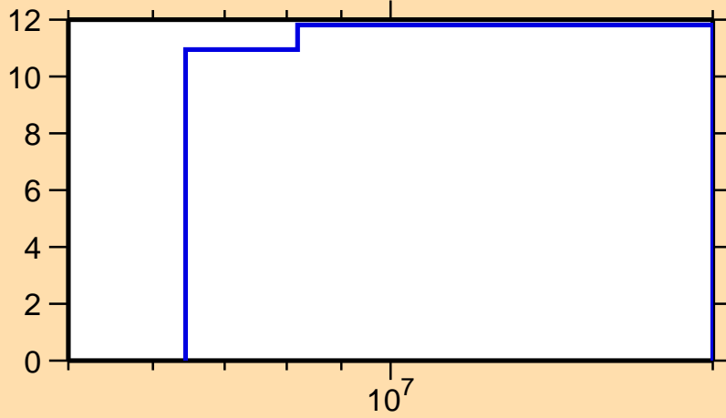
\Delta\sigma/\sigma vs. E for ^{25}\text{Mg}(n,2n)
