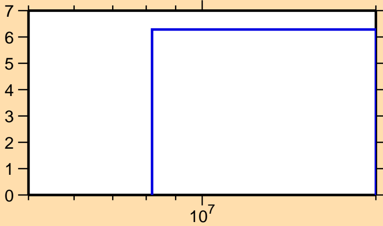
\Delta\sigma/\sigma vs. E for ^{24}\text{Mg}(n,2n)
