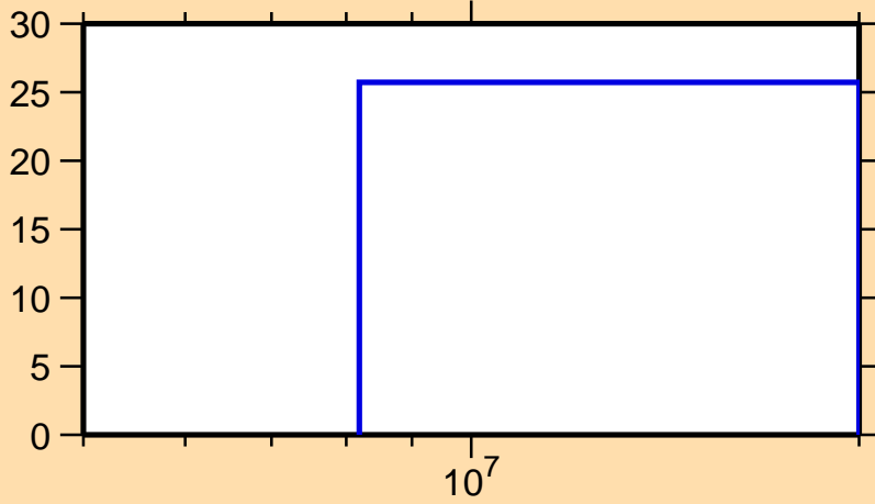
\Delta\sigma/\sigma vs. E for ^{11}\text{B}(n,2n)
