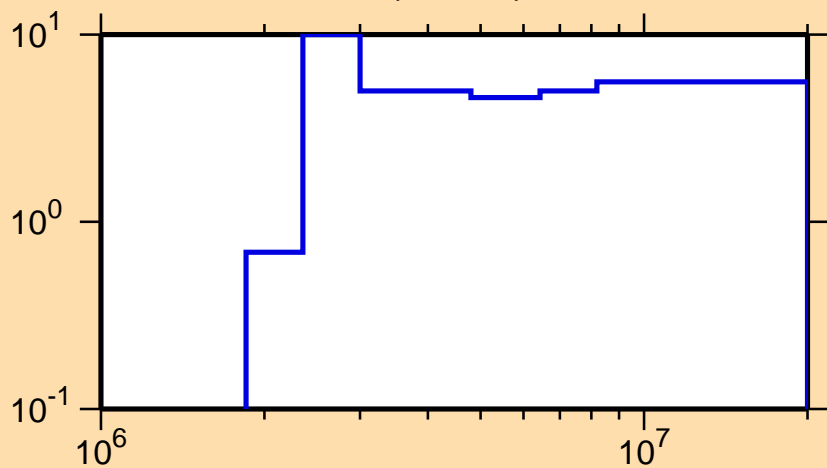
\Delta\sigma/\sigma vs. E for ^{11}\text{B}(n,\text{inel.})
