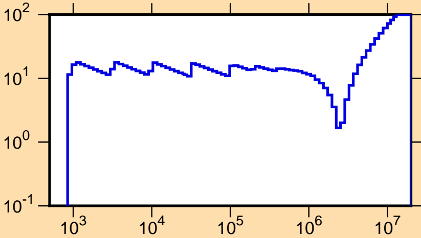
\Delta\phi/\phi vs. E for ^{255}\text{Fm}(n,f)
