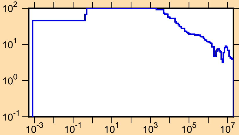
\Delta\sigma/\sigma vs. E for ^{255}\text{Fm}(n,\text{tot.})
