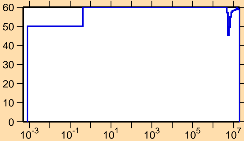
\Delta\sigma/\sigma vs. E for ^{255}\text{Fm}(n,\gamma)
