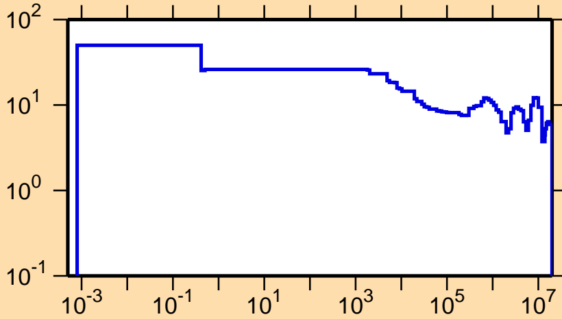
\Delta\sigma/\sigma vs. E for ^{255}\text{Fm}(n,\text{el.})
