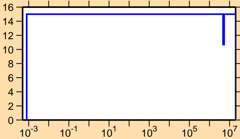
\Delta v/v vs. E for ^{255}\text{Fm} (delayed \nu )
