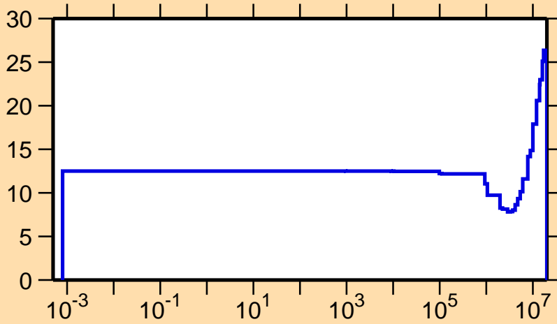
\Delta v/v vs. E for ^{255}\text{Fm} (prompt \nu )
