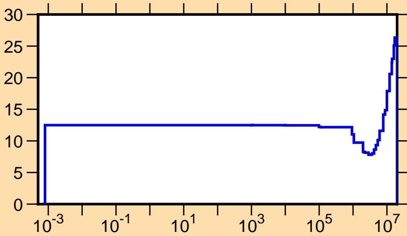
\Delta v/v vs. E for ^{255}\text{Fm} (total \nu )
