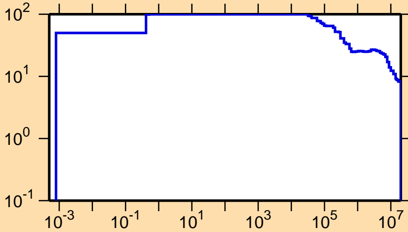
\Delta\sigma/\sigma vs. E for ^{255}\text{Fm}(n,f)
