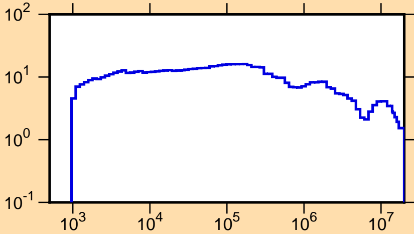
\Delta\mu/\mu vs. E for ^{255}\text{Fm} (mt251)
