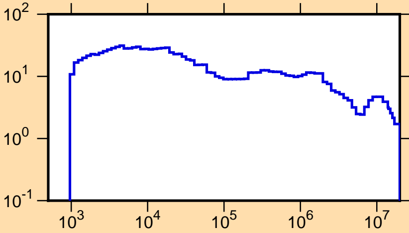
\Delta\mu/\mu vs. E for ^{254}\text{Es}(\text{mt251})
