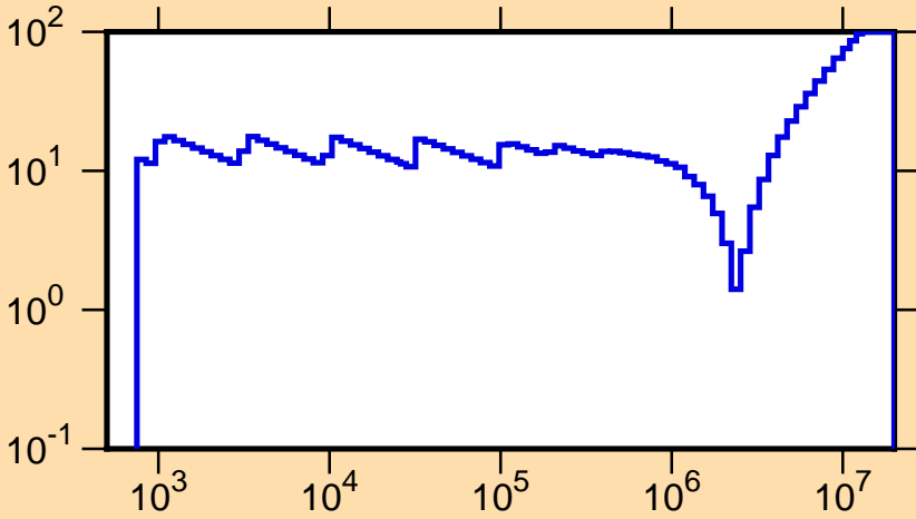
\Delta\phi/\phi vs. E for ^{254}\text{Es}(n,f)
