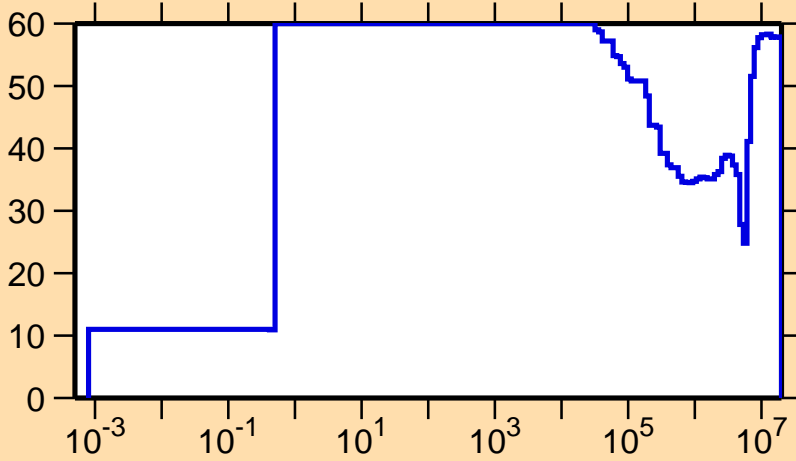
\Delta\sigma/\sigma vs. E for ^{254}\text{Es}(n,\gamma)
