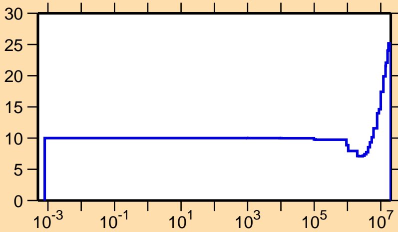
\Delta v/v vs. E for ^{254}\text{Es} (prompt \nu )
