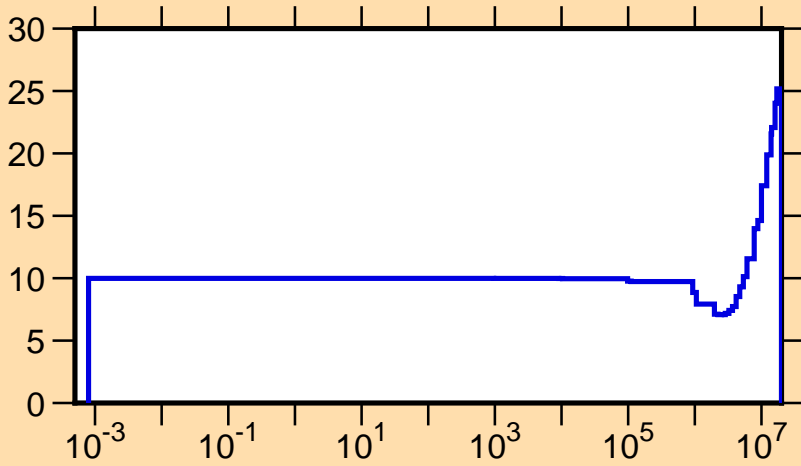
\Delta v/v vs. E for ^{254}\text{Es} (total \nu )
