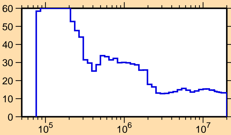
\Delta\sigma/\sigma vs. E for ^{254}\text{Es}(n,\text{inel.})
