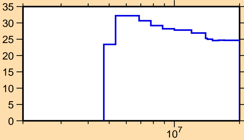
\Delta\sigma/\sigma vs. E for ^{254}\text{Es}(n,2n)
