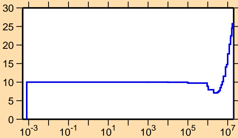
\Delta v/v vs. E for ^{252}\text{Es} (prompt \nu )
