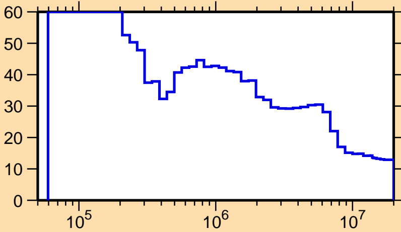
\Delta\sigma/\sigma vs. E for ^{252}\text{Es}(n,\text{inel.})
