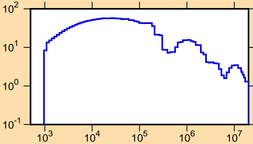
\Delta\mu/\mu vs. E for ^{254}\text{Cf}(\text{mt251})
