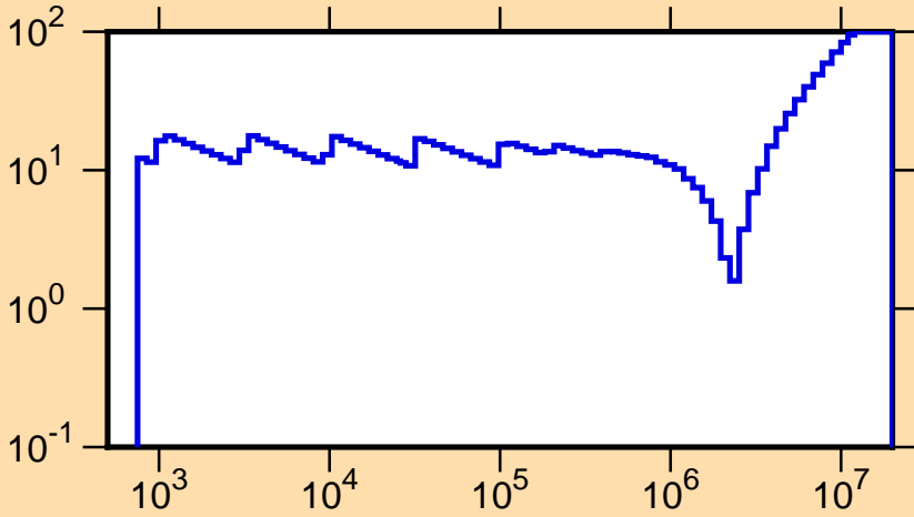
\Delta\phi/\phi vs. E for ^{254}\text{Cf}(n,f)
