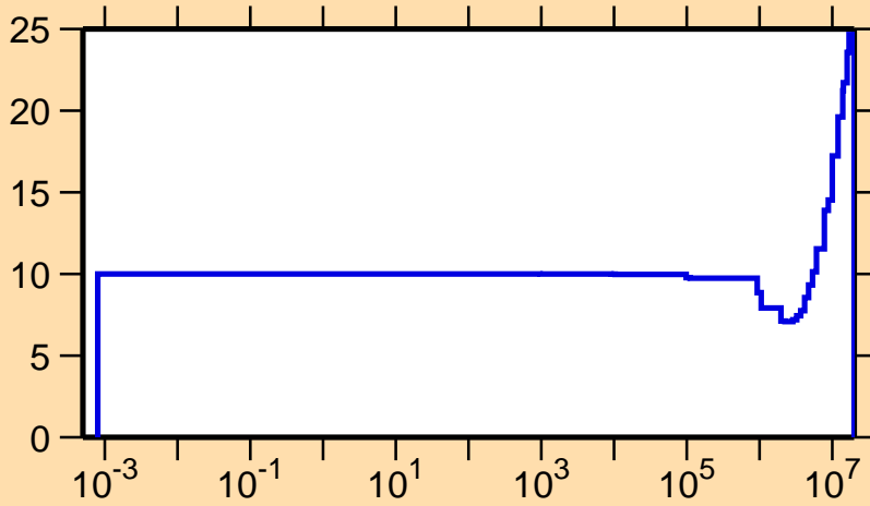
\Delta v/v vs. E for ^{254}\text{Cf}(\text{prompt } \nu)
