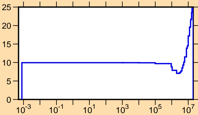
\Delta v/v vs. E for ^{254}\text{Cf}(\text{total } \nu)
