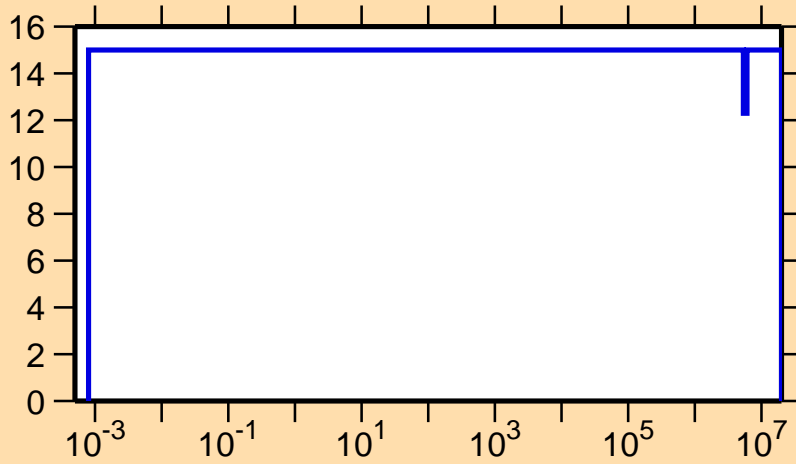
\Delta v/v vs. E for ^{254}\text{Cf}(\text{delayed } \nu)
