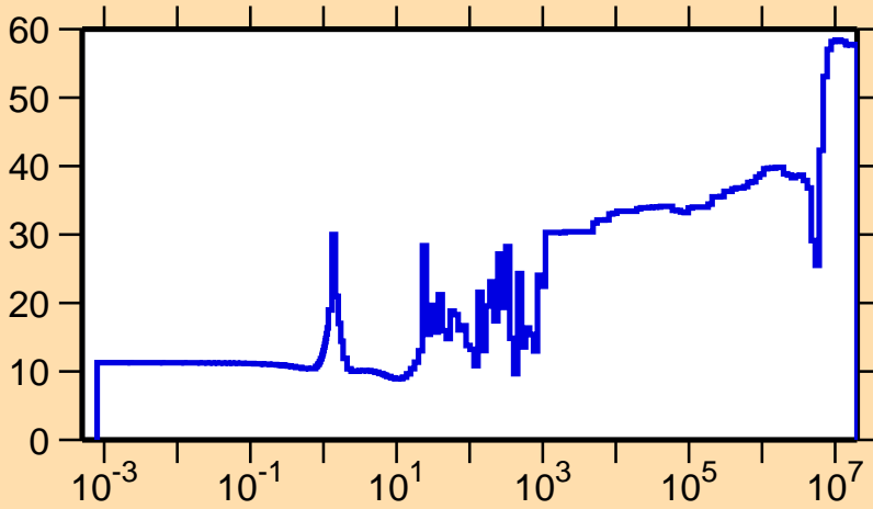
\Delta\sigma/\sigma vs. E for ^{252}\text{Cf}(n,\gamma)
