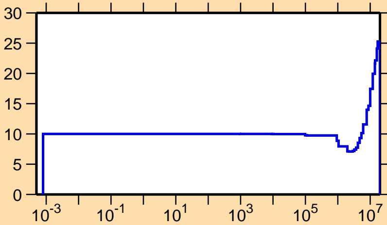
\Delta v/v vs. E for ^{252}\text{Cf}(\text{prompt } \nu)
