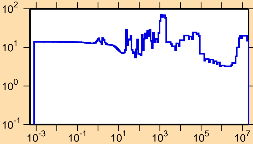
\Delta\sigma/\sigma vs. E for ^{252}\text{Cf}(n,f)
