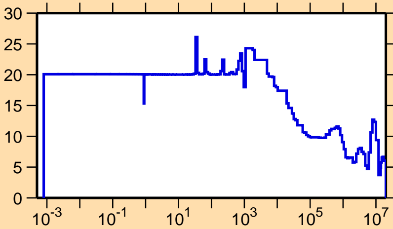
\Delta\sigma/\sigma vs. E for ^{252}\text{Cf}(n,\text{el.})
