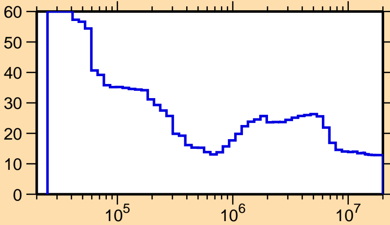
\Delta\sigma/\sigma vs. E for ^{251}\text{Cf}(n,\text{inel.})
