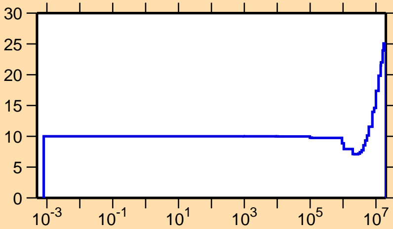
\Delta v/v vs. E for ^{250}\text{Cf} (prompt \nu )
