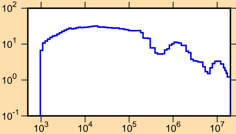
\Delta\mu/\mu vs. E for ^{250}\text{Cf}(\text{mt251})
