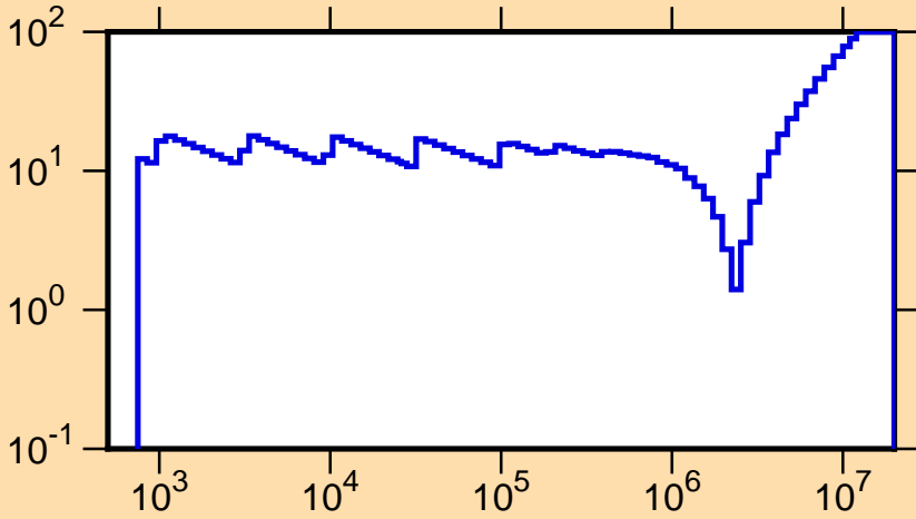
\Delta\phi/\phi vs. E for ^{250}\text{Cf}(n,f)
