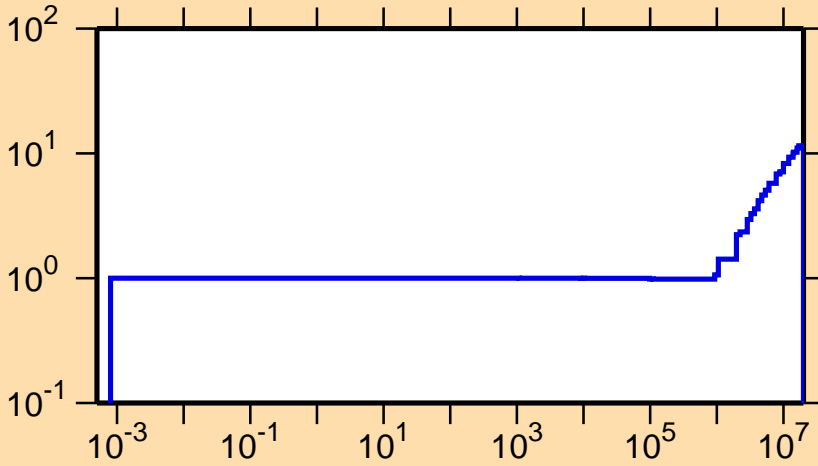
\Delta v/v vs. E for ^{249}\text{Cf} (prompt \nu )
