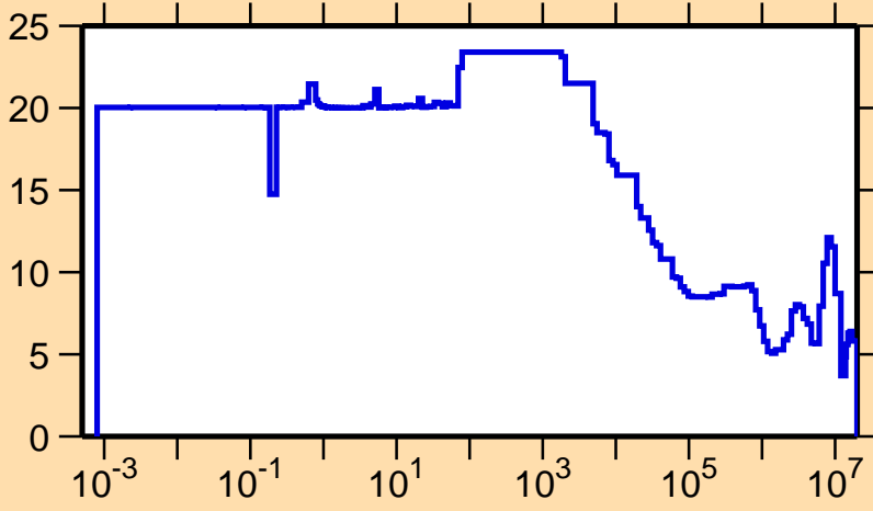
\Delta\sigma/\sigma vs. E for ^{249}\text{Cf}(n,\text{el.})
