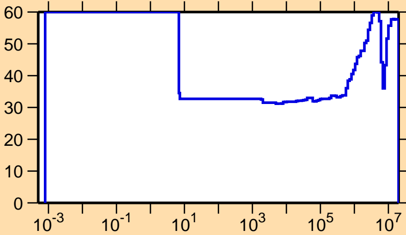
\Delta\sigma/\sigma vs. E for ^{248}\text{Cf}(n,\gamma)
