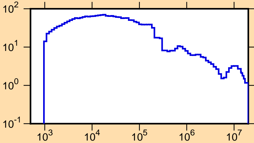
\Delta\mu/\mu vs. E for ^{248}\text{Cf}(\text{mt251})
