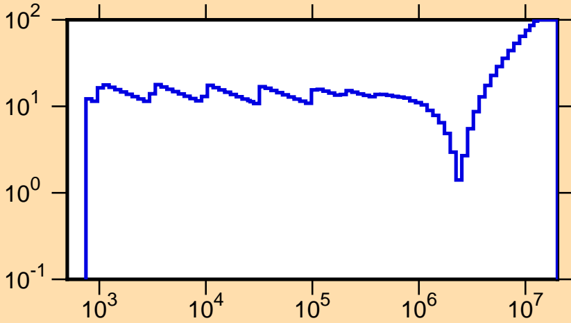
\Delta\phi/\phi vs. E for ^{248}\text{Cf}(n,f)
