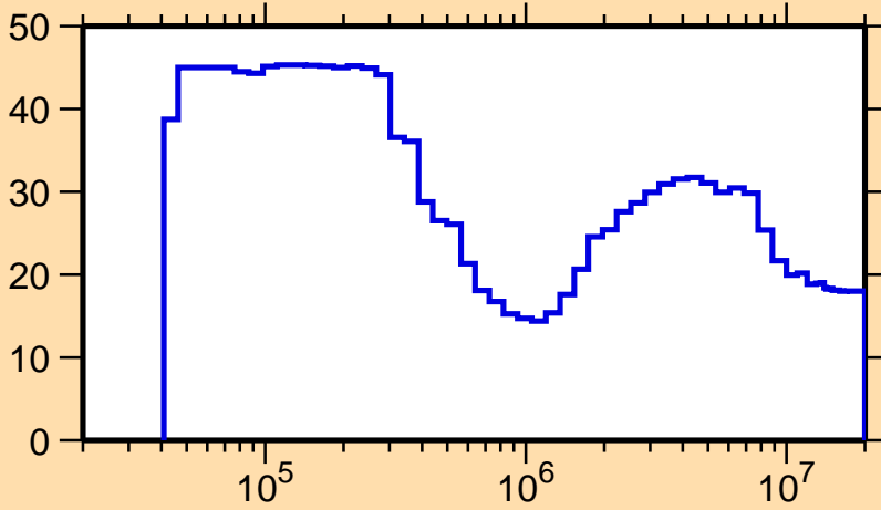
\Delta\sigma/\sigma vs. E for ^{248}\text{Cf}(n,\text{inel.})
