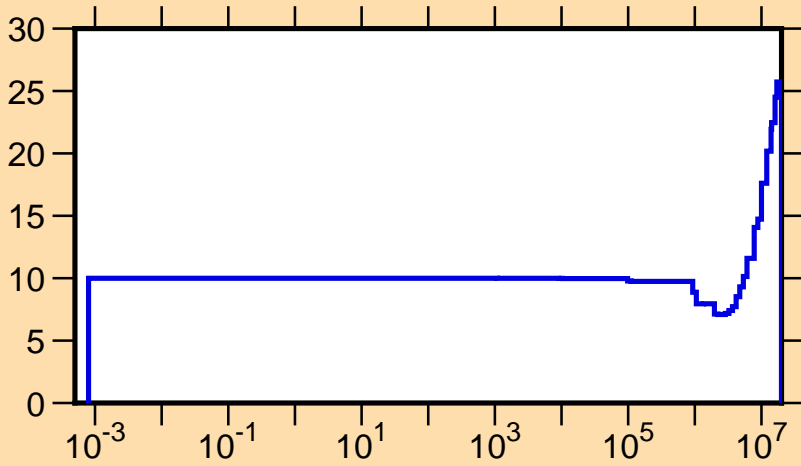
\Delta v/v vs. E for ^{248}\text{Cf}(\text{total } \nu)
