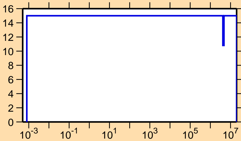
\Delta v/v vs. E for ^{248}\text{Cf}(\text{delayed } \nu)
