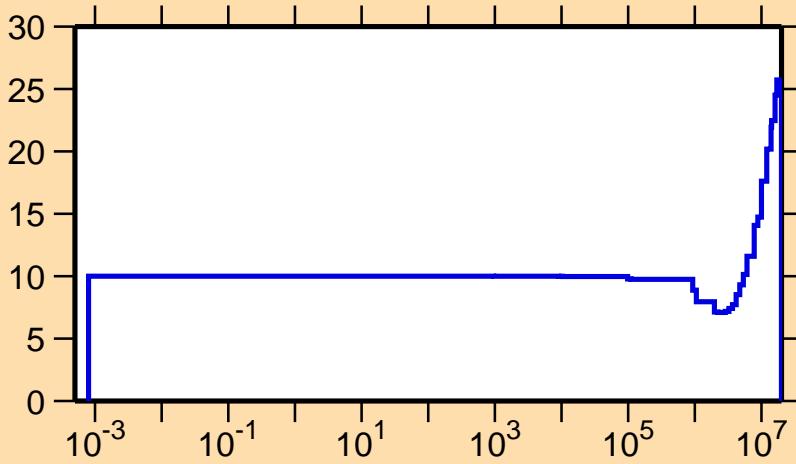
\Delta v/v vs. E for ^{248}\text{Cf}(\text{prompt } \nu)
