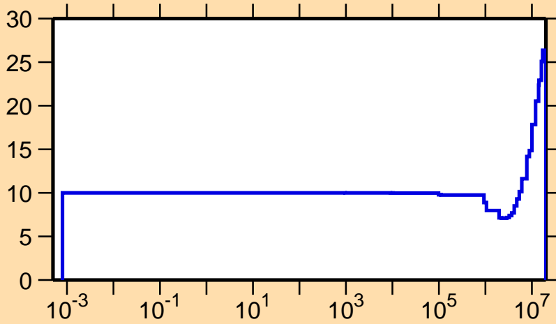
\Delta v/v vs. E for ^{246}\text{Cf}(\text{prompt } \nu)
