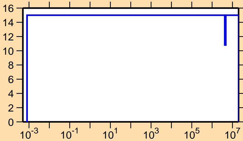
\Delta v/v vs. E for ^{246}\text{Cf}(\text{delayed } \nu)
