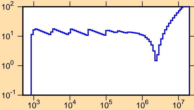
\Delta\phi/\phi vs. E for ^{246}\text{Cf}(n,f)
