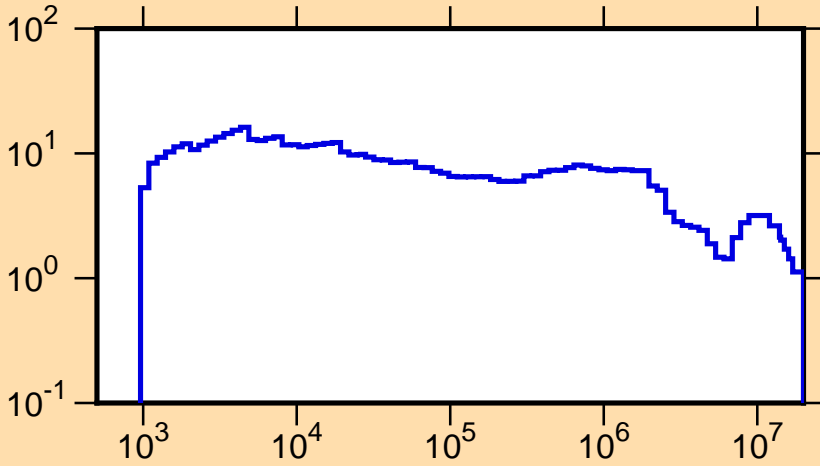
\Delta\mu/\mu vs. E for ^{246}\text{Cf}(\text{mt251})
