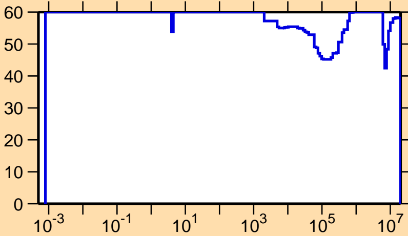
\Delta\sigma/\sigma vs. E for ^{246}\text{Cf}(n,\gamma)
