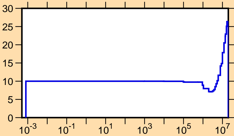
\Delta v/v vs. E for ^{246}\text{Cf}(\text{total } \nu)
