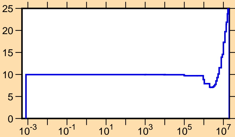
\Delta v/v vs. E for ^{250}\text{Bk}(\text{total } \nu)
