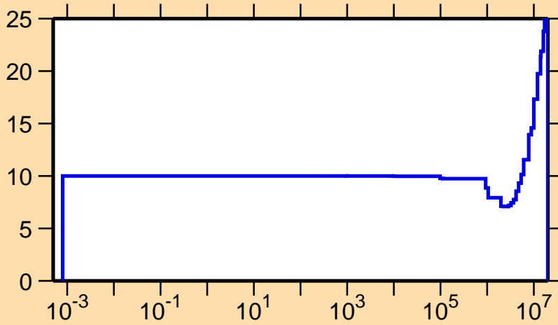
\Delta v/v vs. E for ^{250}\text{Bk}(\text{prompt } \nu)
