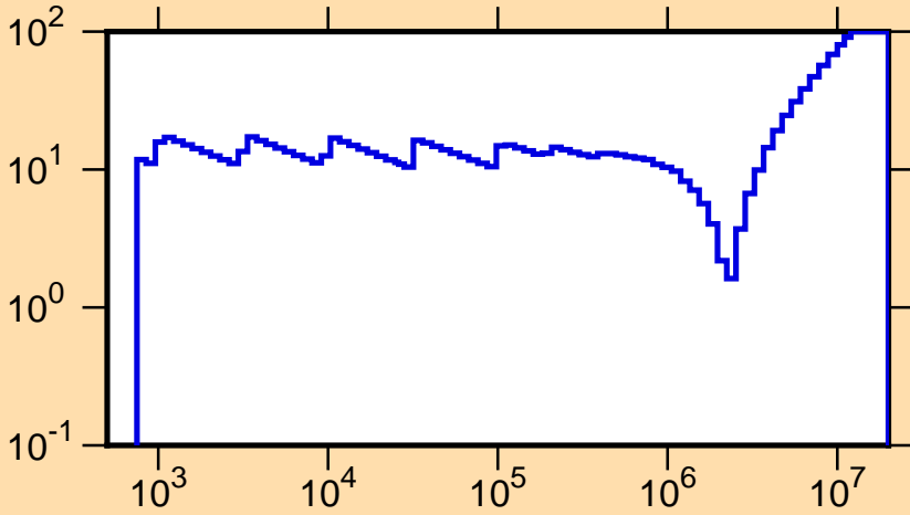
\Delta\phi/\phi vs. E for ^{250}\text{Bk}(n,f)
