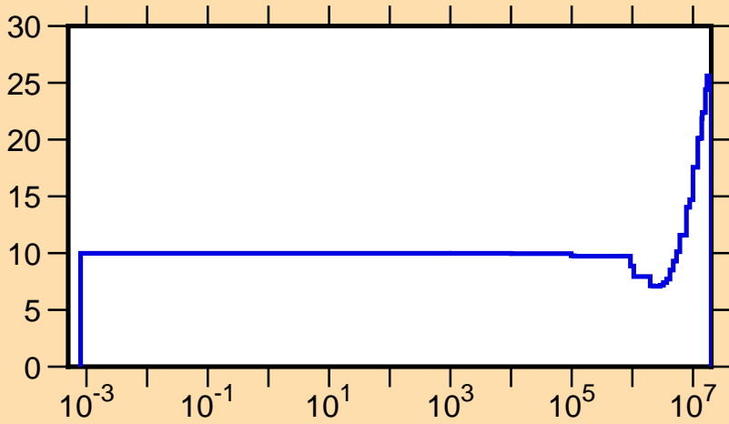
\Delta v/v vs. E for ^{248}\text{Bk}(\text{total } \nu)
