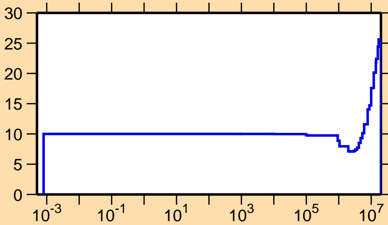
\Delta v/v vs. E for ^{248}\text{Bk} (prompt \nu )
