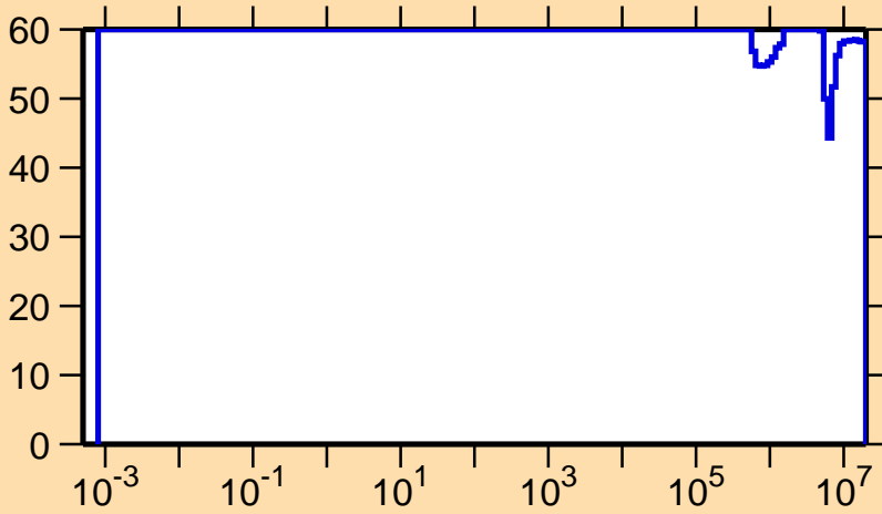
\Delta\sigma/\sigma vs. E for ^{248}\text{Bk}(n,\gamma)
