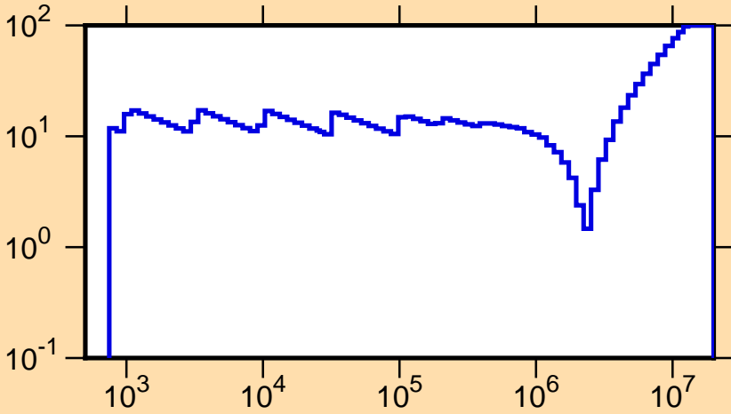
\Delta\phi/\phi vs. E for ^{248}\text{Bk}(n,f)
