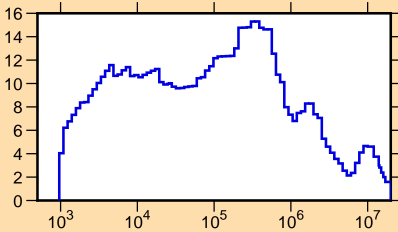
\Delta\mu/\mu vs. E for ^{248}\text{Bk}(\text{mt251})
