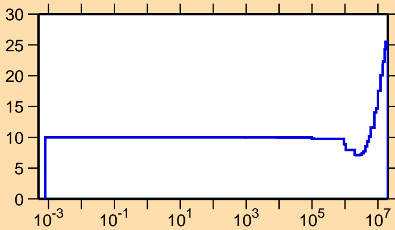
\Delta v/v vs. E for ^{247}\text{Bk} (prompt \nu )
