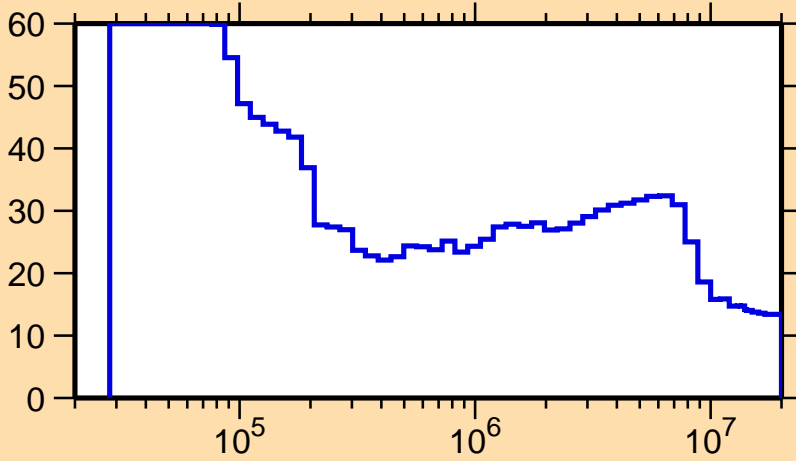
\Delta\sigma/\sigma vs. E for ^{247}\text{Bk}(n,\text{inel.})
