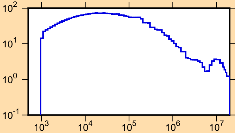
\Delta\mu/\mu vs. E for ^{245}\text{Bk}(\text{mt251})
