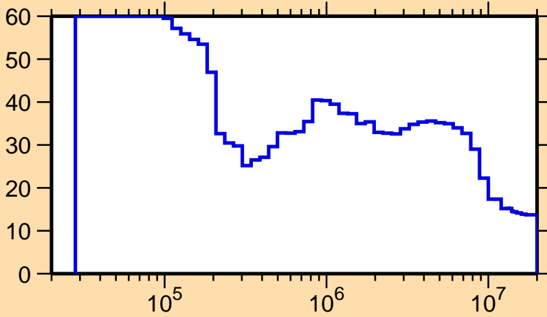
\Delta\sigma/\sigma vs. E for ^{245}\text{Bk}(n,\text{inel.})
