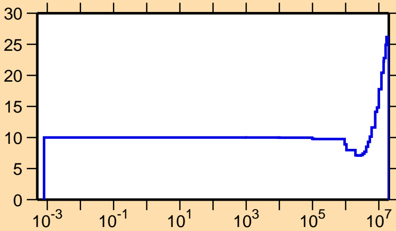
\Delta v/v vs. E for ^{245}\text{Bk}(\text{prompt } \nu)
