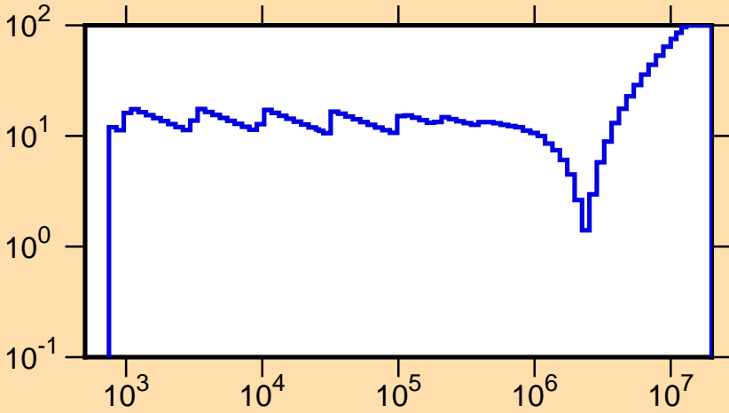
\Delta\phi/\phi vs. E for ^{245}\text{Bk}(n,f)
