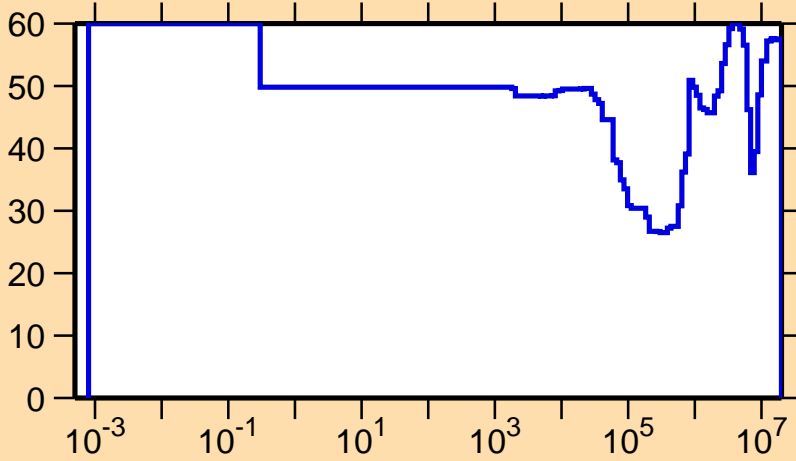
\Delta\sigma/\sigma vs. E for ^{245}\text{Bk}(n,\gamma)
