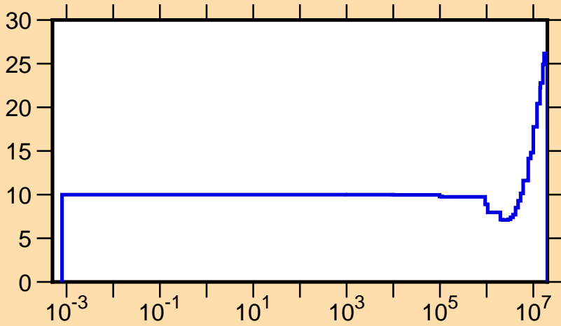
\Delta v/v vs. E for ^{245}\text{Bk}(\text{total } \nu)
