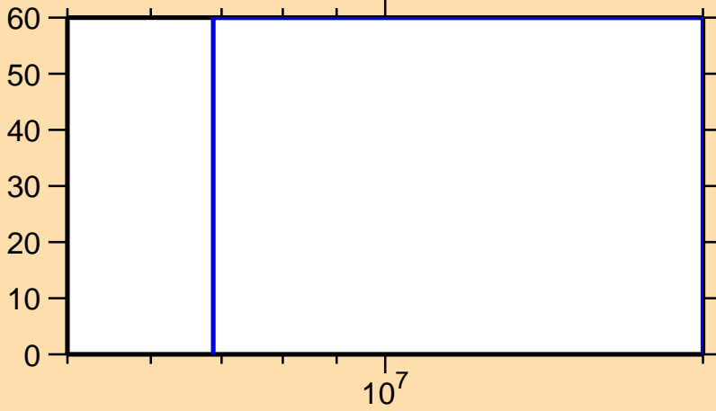
\Delta\sigma/\sigma vs. E for ^{245}\text{Bk}(n,2n)
