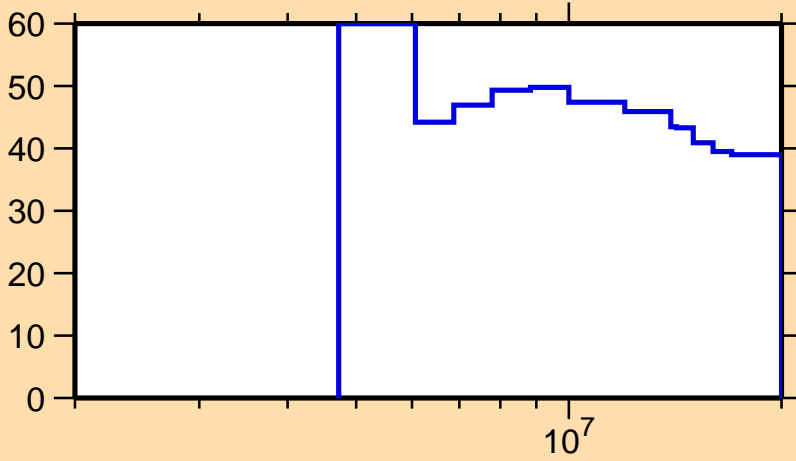
\Delta\sigma/\sigma vs. E for ^{249}\text{Cm}(n,2n)
