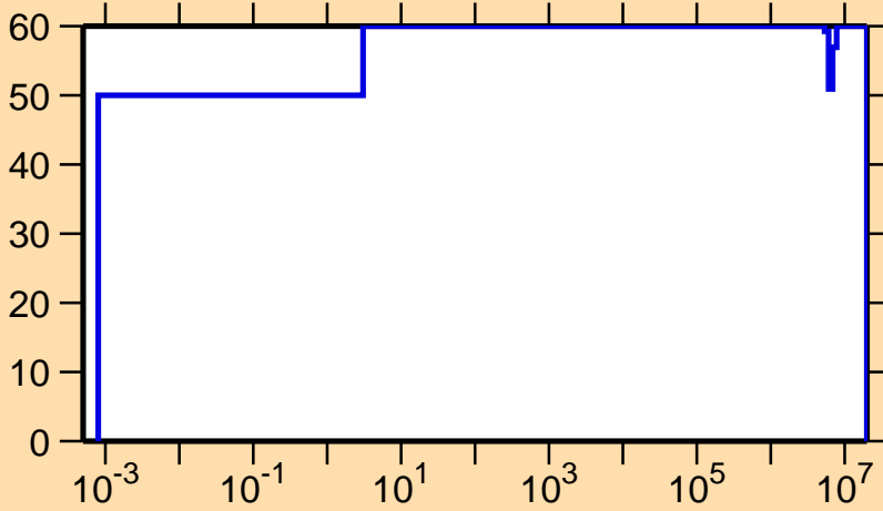
\Delta\sigma/\sigma vs. E for ^{249}\text{Cm}(n,\gamma)
