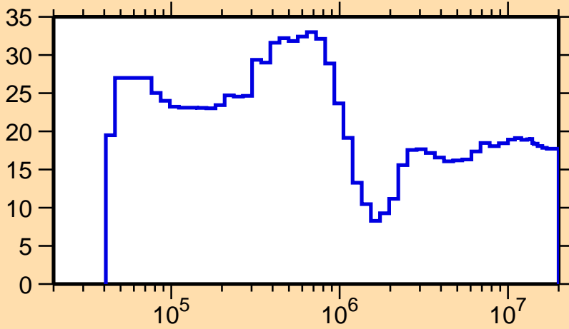
\Delta\sigma/\sigma vs. E for ^{246}\text{Cm}(n,\text{inel.})
