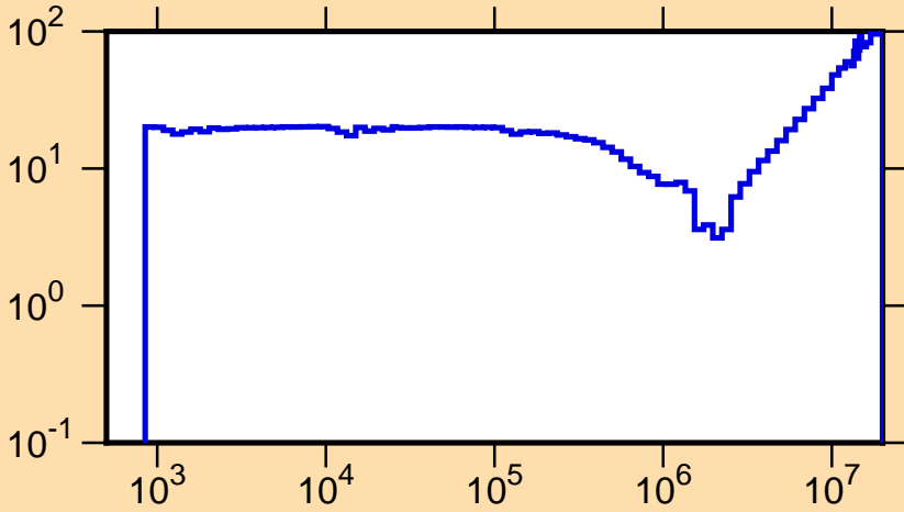
\Delta\phi/\phi vs. E for ^{246}\text{Cm}(n,f)
