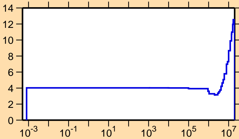
\Delta v/v vs. E for ^{246}\text{Cm} (prompt \nu )
