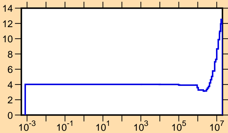
\Delta v/v vs. E for ^{246}\text{Cm} (total \nu )
