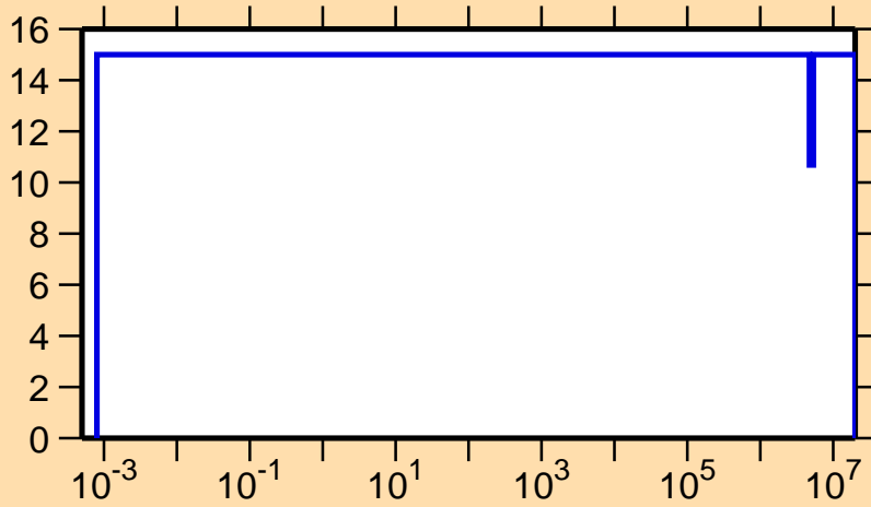
\Delta\nu/\nu vs. E for ^{246}\text{Cm} (delayed \nu )
