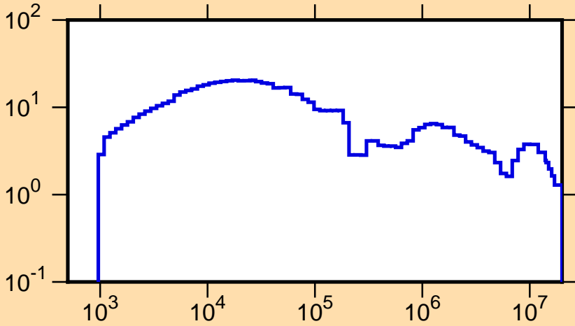
\Delta\mu/\mu vs. E for ^{246}\text{Cm}(\text{mt251})
