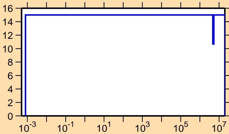
\Delta v/v vs. E for ^{245}\text{Cm} (delayed \nu )
