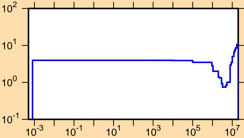
\Delta v/v vs. E for ^{245}\text{Cm} (total \nu )
