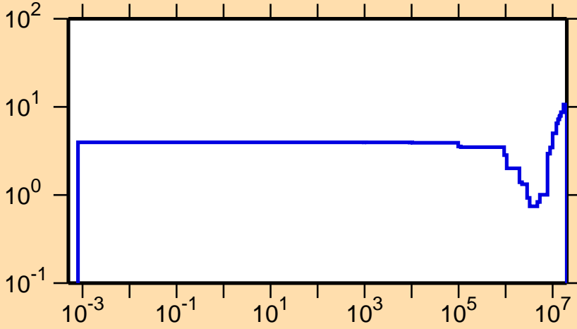
\Delta v/v vs. E for ^{245}\text{Cm} (prompt \nu )
