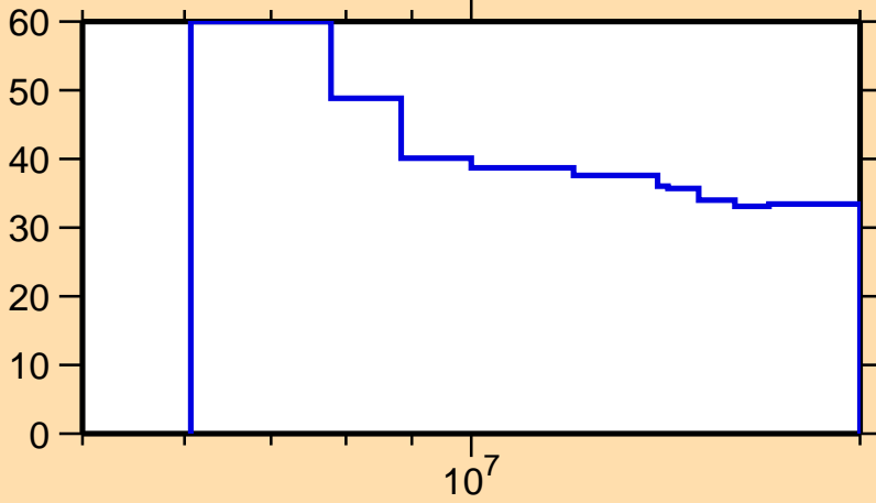
\Delta\sigma/\sigma vs. E for ^{244}\text{Cm}(n,2n)
