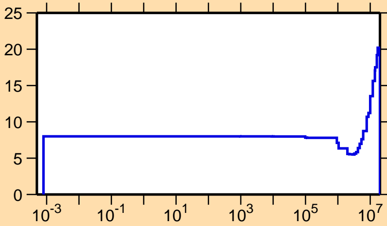
\Delta v/v vs. E for ^{244}\text{Cm} (prompt \nu )
