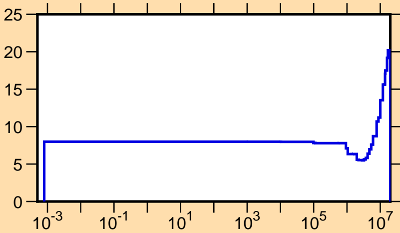
\Delta v/v vs. E for ^{244}\text{Cm}(\text{total } \nu)
