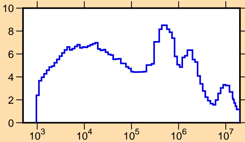
\Delta\mu/\mu vs. E for ^{243}\text{Cm}(\text{mt251})
