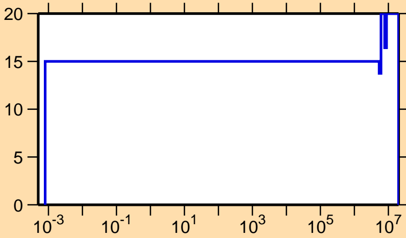
\Delta v/v vs. E for ^{243}\text{Cm}(\text{delayed } \nu)
