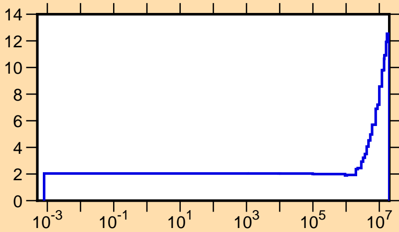
\Delta v/v vs. E for ^{243}\text{Cm} (total \nu )
