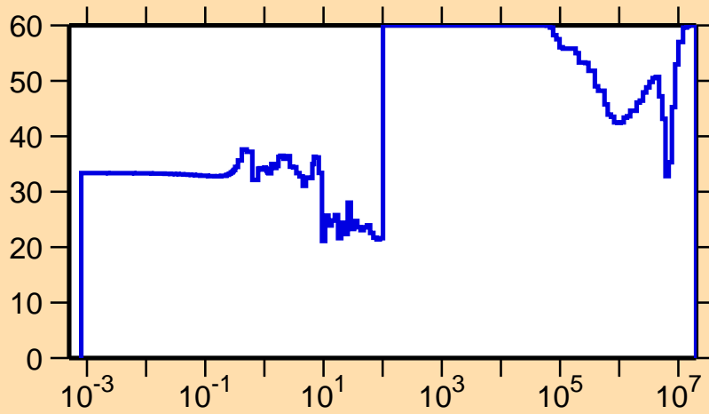
\Delta\sigma/\sigma vs. E for ^{243}\text{Cm}(n,\gamma)
