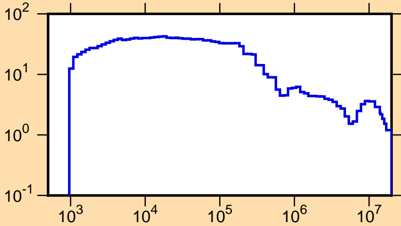
\Delta\mu/\mu vs. E for ^{242}\text{Cm}(\text{mt251})
