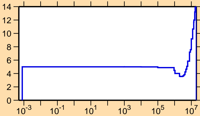
\Delta v/v vs. E for ^{242}\text{Cm} (prompt \nu )
