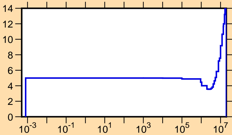
\Delta v/v vs. E for ^{242}\text{Cm} (total \nu )
