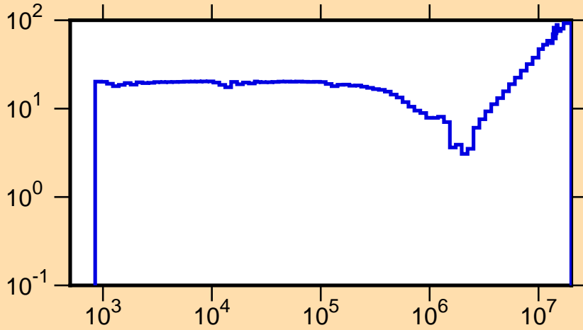
\Delta\phi/\phi vs. E for ^{242}\text{Cm}(n,f)
