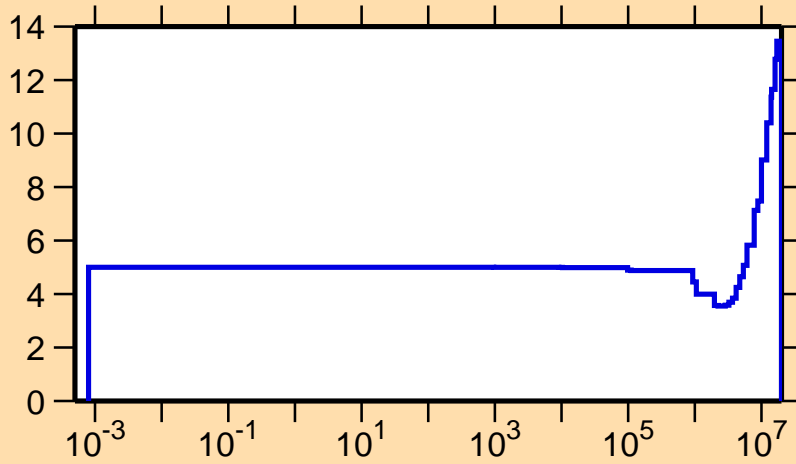
\Delta v/v vs. E for ^{240}\text{Cm} (prompt \nu )
