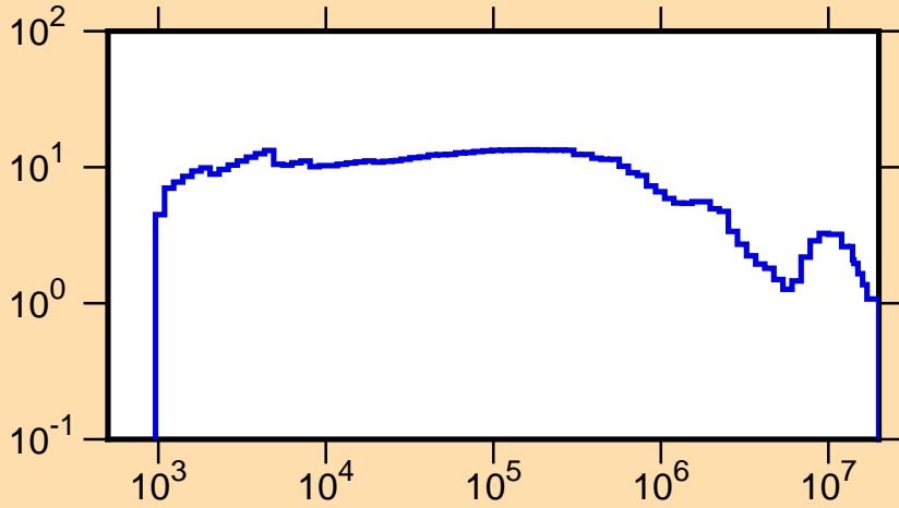
\Delta\mu/\mu vs. E for ^{240}\text{Cm}(\text{mt251})
