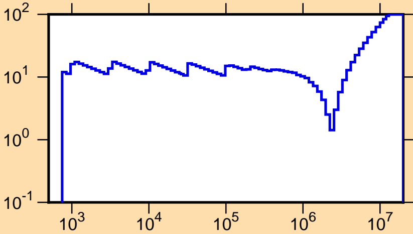
\Delta\phi/\phi vs. E for ^{240}\text{Cm}(n,f)
