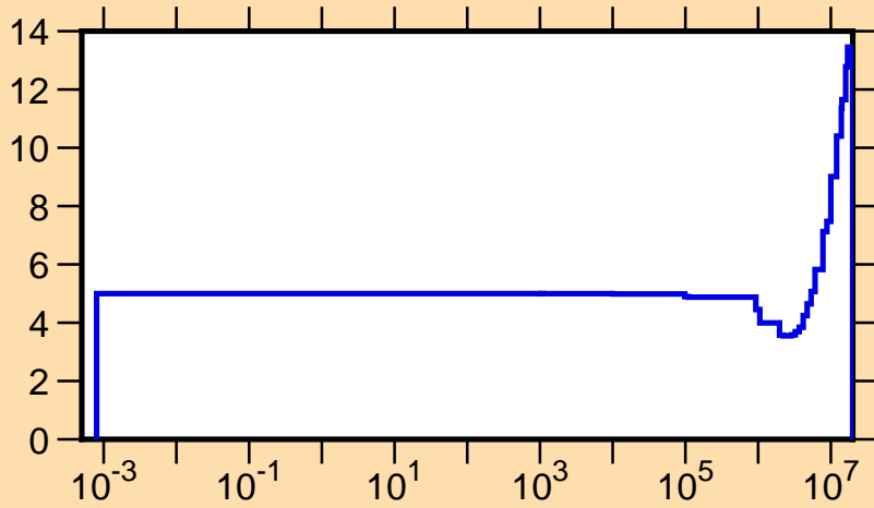
\Delta v/v vs. E for ^{240}\text{Cm} (total \nu )
