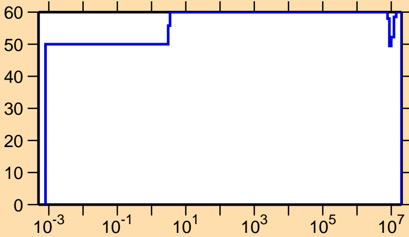
\Delta\sigma/\sigma vs. E for ^{240}\text{Cm}(n,\gamma)
