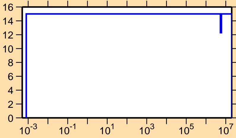
\Delta\nu/\nu vs. E for ^{240}\text{Am} (delayed \nu )
