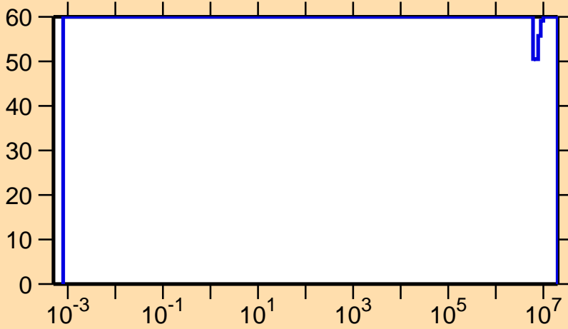
\Delta\sigma/\sigma vs. E for ^{240}\text{Am}(n,\gamma)
