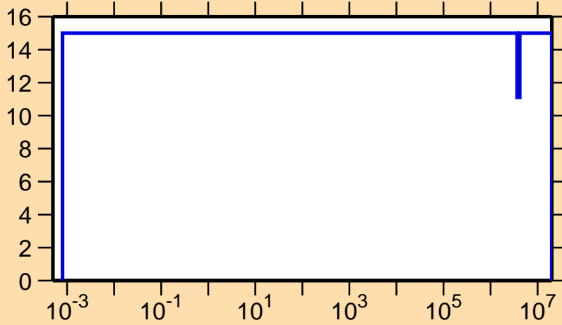
\Delta v/v vs. E for ^{237}\text{Pu}(\text{delayed } \nu)
