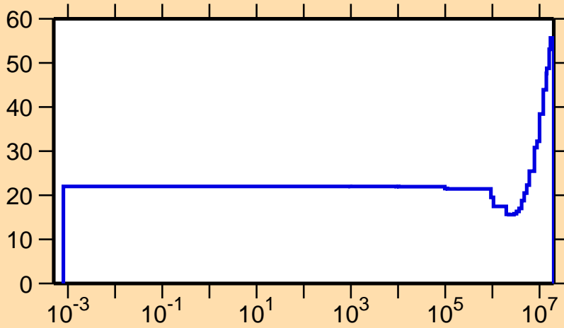
\Delta v/v vs. E for ^{238}\text{Np} (prompt \nu )
