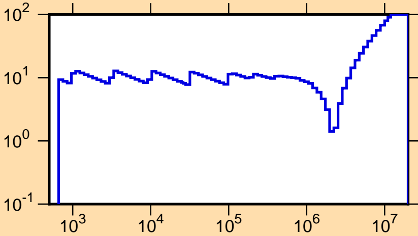
\Delta\phi/\phi vs. E for ^{238}\text{Np}(n,f)
