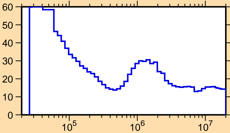
\Delta\sigma/\sigma vs. E for ^{238}\text{Np}(n,\text{inel.})
