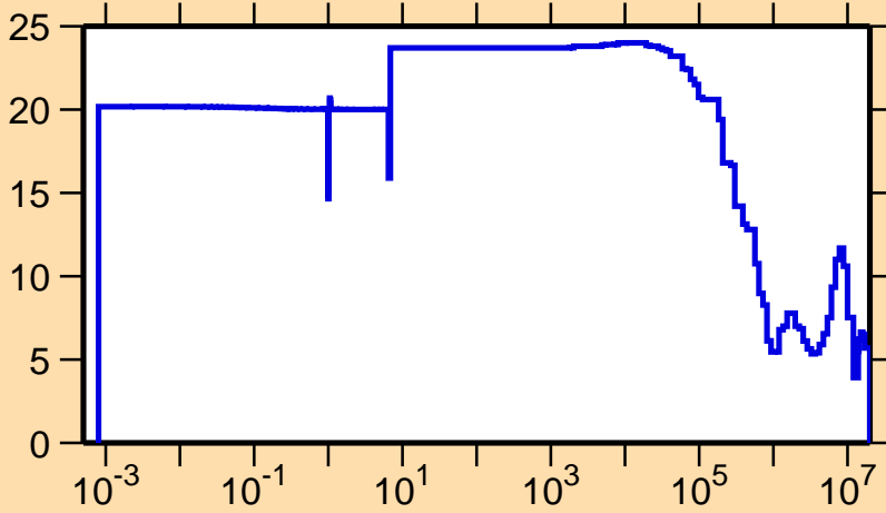
\Delta\sigma/\sigma vs. E for ^{238}\text{Np}(n,\text{el.})
