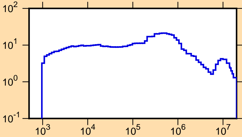
\Delta\mu/\mu vs. E for ^{238}\text{Np}(\text{mt251})
