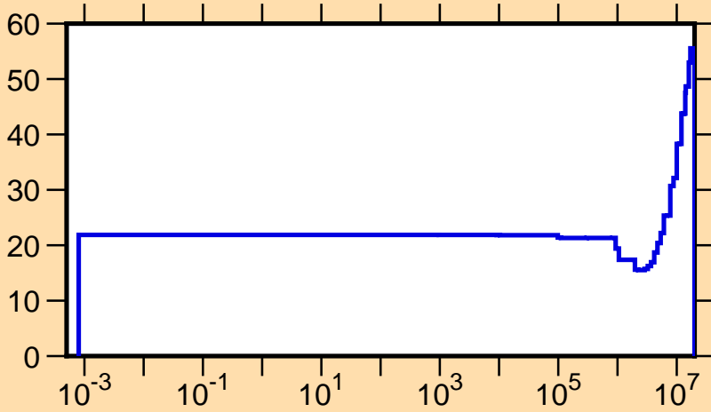
\Delta v/v vs. E for ^{238}\text{Np} (total v )
