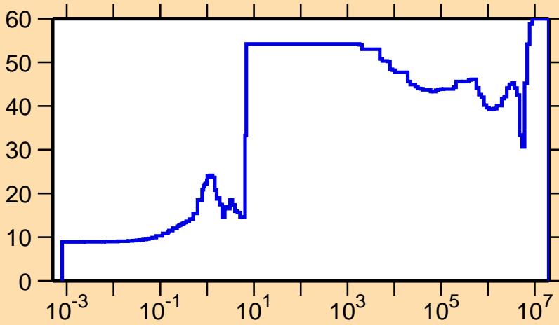
\Delta\sigma/\sigma vs. E for ^{238}\text{Np}(n,\gamma)
