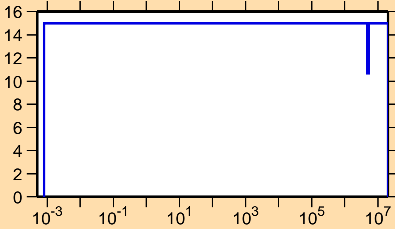
\Delta v/v vs. E for ^{235}\text{Np}(\text{delayed } \nu)
