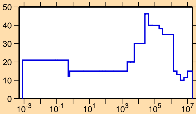
\Delta\sigma/\sigma vs. E for ^{234}\text{U}(n,f)
