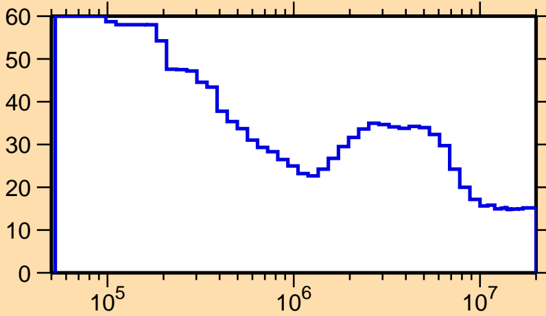
\Delta\sigma/\sigma vs. E for ^{230}\text{U}(n,\text{inel.})
