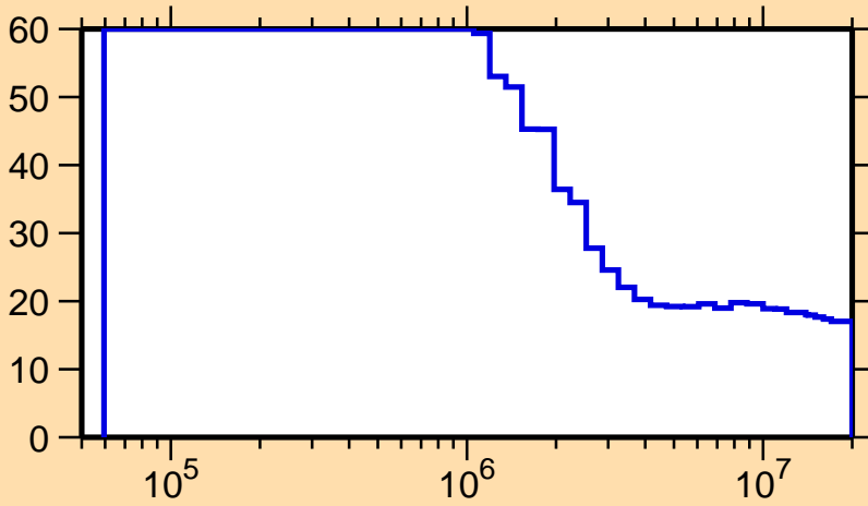
\Delta\sigma/\sigma vs. E for ^{232}\text{Pa}(n,\text{inel.})
